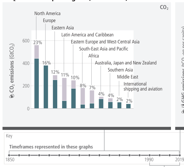
a) Historical cumulative net anthropogenic CO 2 emissions per region (1850–2019)
