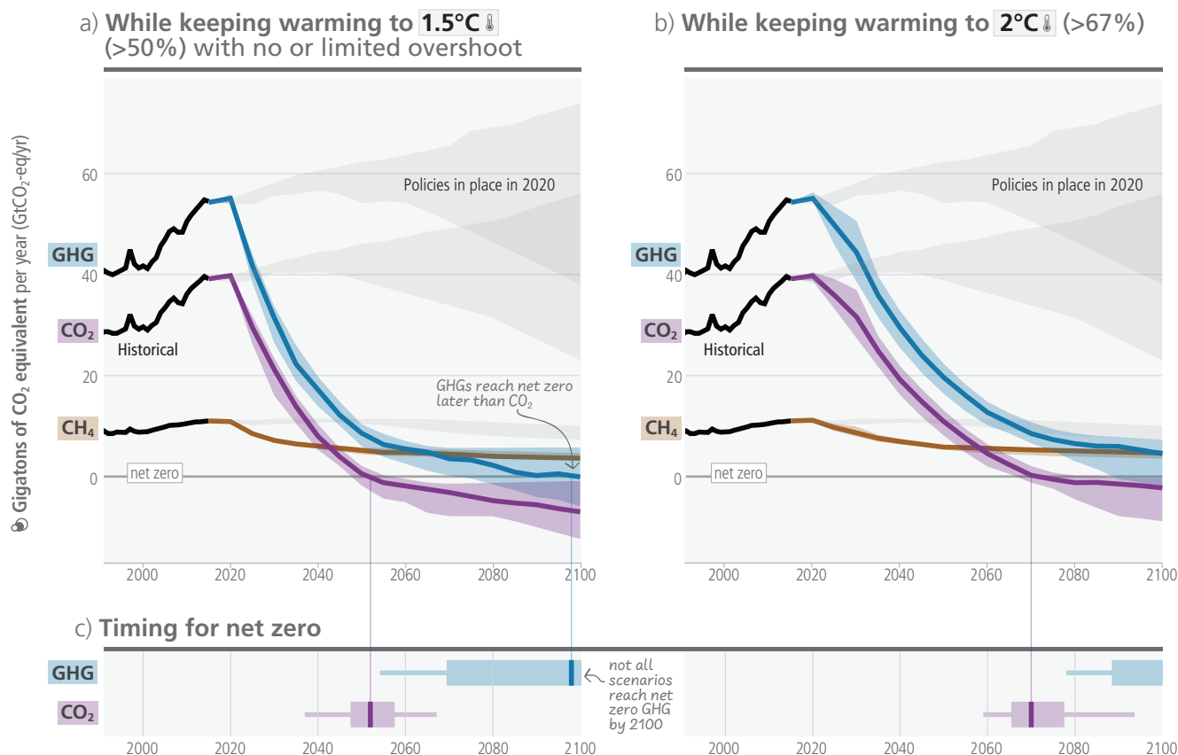
Figure 3.6: Total GHG, CO 2 and CH 4 emissions and timing of reaching net zero in different mitigation pathways. Top row: GHG, CO 2 and CH 4 emissions over time (in GtCO 2 -eq) with historical emissions, projected emissions in line with policies implemented until the end of 2020 (grey), and pathways consistent with temperature goals in colour (blue, purple, and brown, respectively). Panel (a) (left) shows pathways that limit warming to 1.5°C (>50%) with no or limited overshoot (C1) and Panel (b) (right) shows pathways that limit warming to 2°C (>67%) (C3). Bottom row: Panel (c) shows median (vertical line), likely (bar) and very likely (thin lines) timing of reaching net zero GHG and CO 2 emissions for global modelled pathways that limit warming to 1.5°C (>50%) with no or limited overshoot (C1) (left) or 2°C (>67%) (C3) (right). [WGIII Figure SPM.5]
